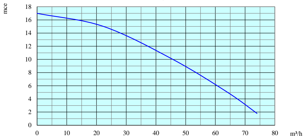
Courbe Q-H
