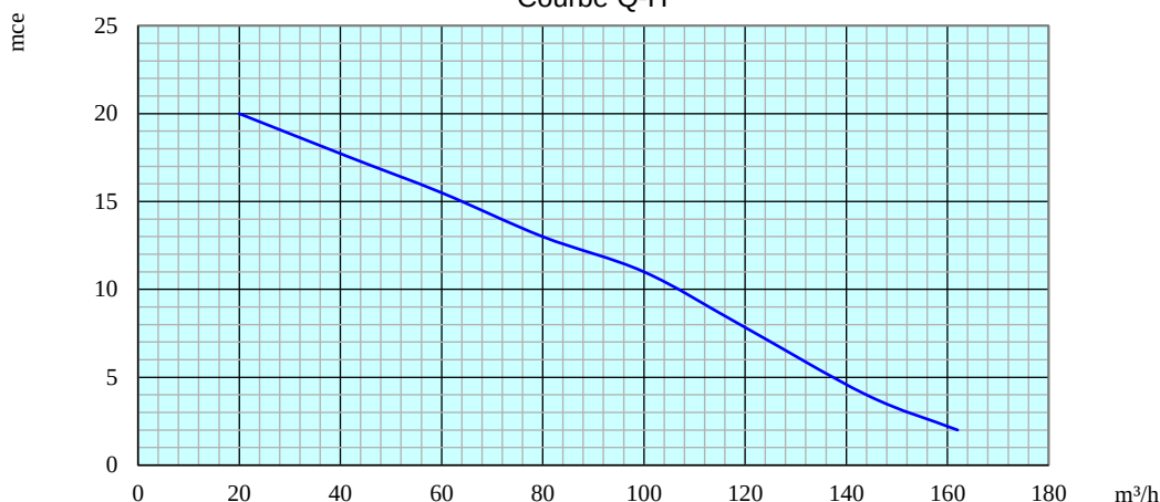
Courbe Q-H
