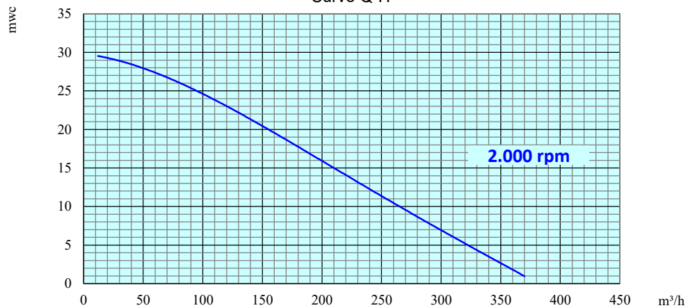
Curve Q-H
