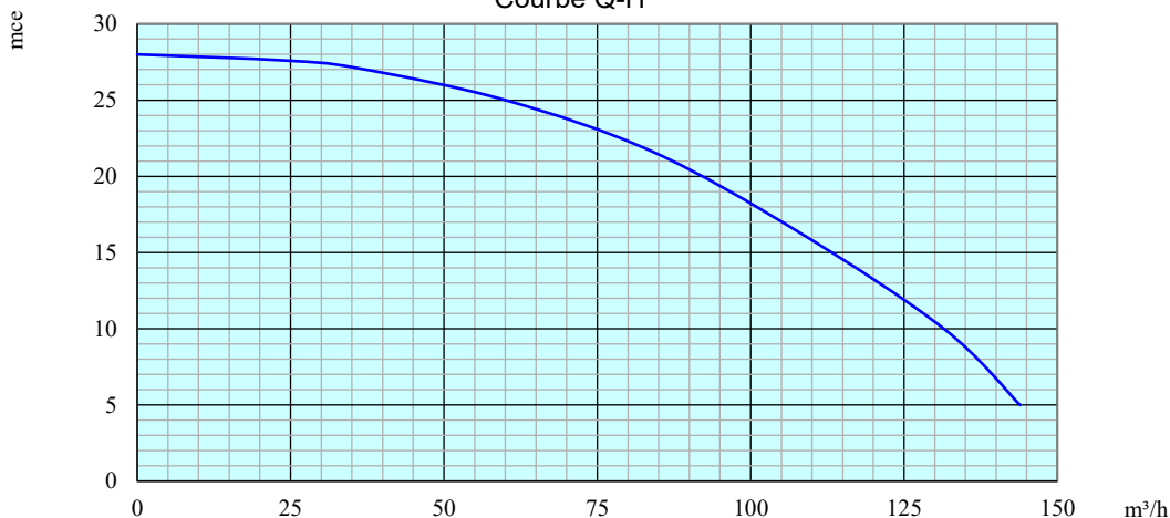
Courbe Q-H
