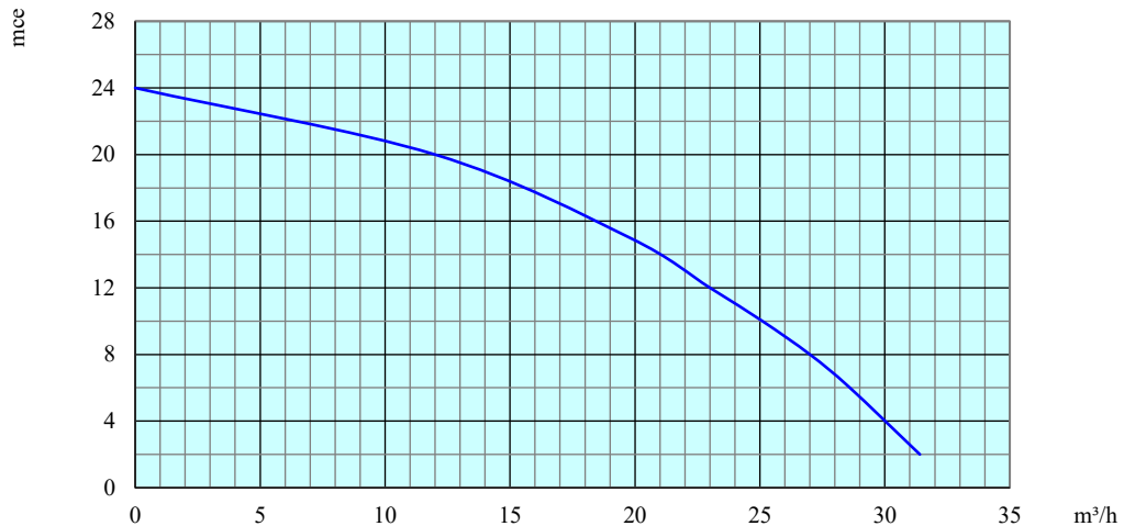
Courbe Q-H
