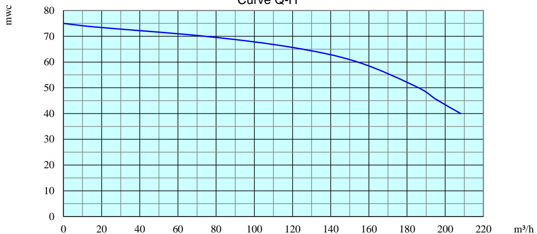
Curve Q-H
