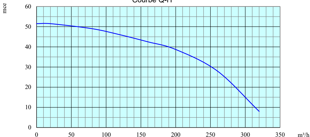
Courbe Q-H
