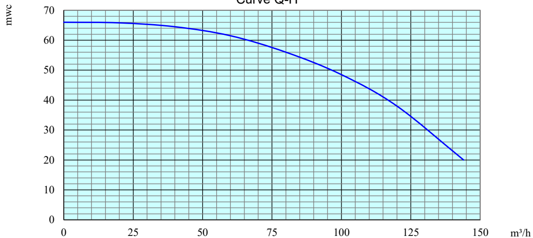
Curve Q-H
