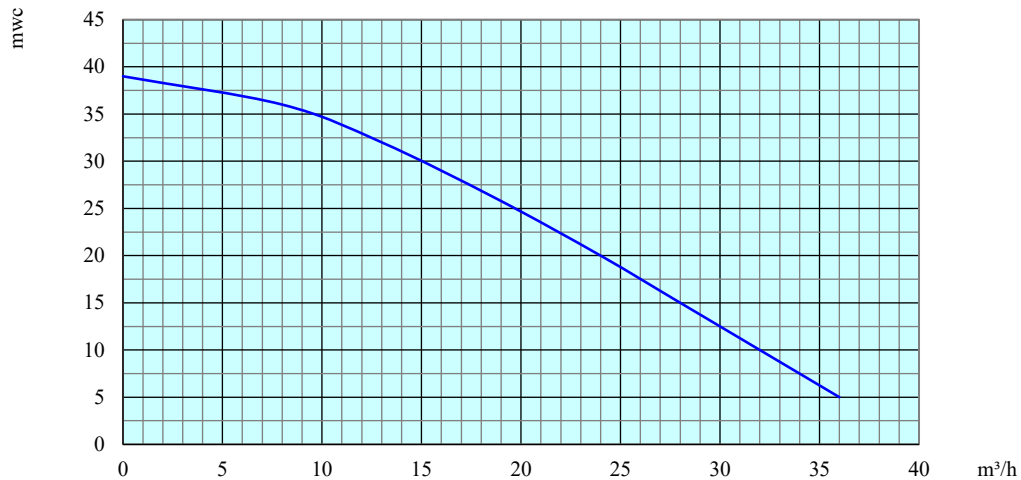
Curve Q-H
