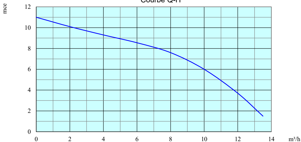
Courbe Q-H
