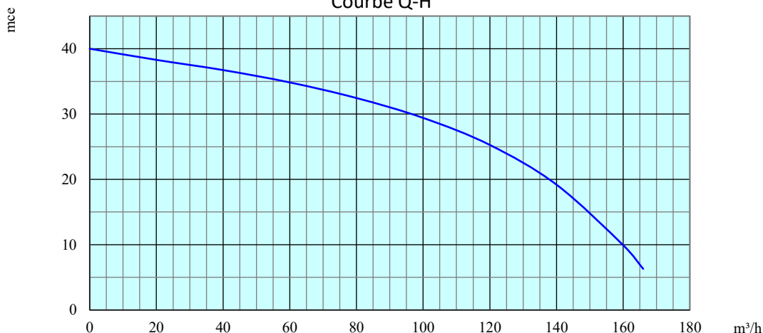
Courbe Q-H
