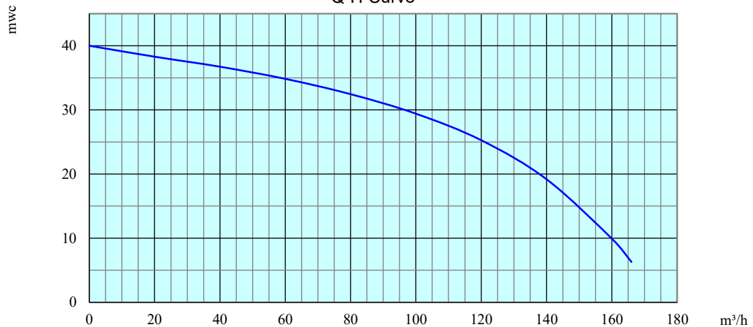
Q-H Curve
