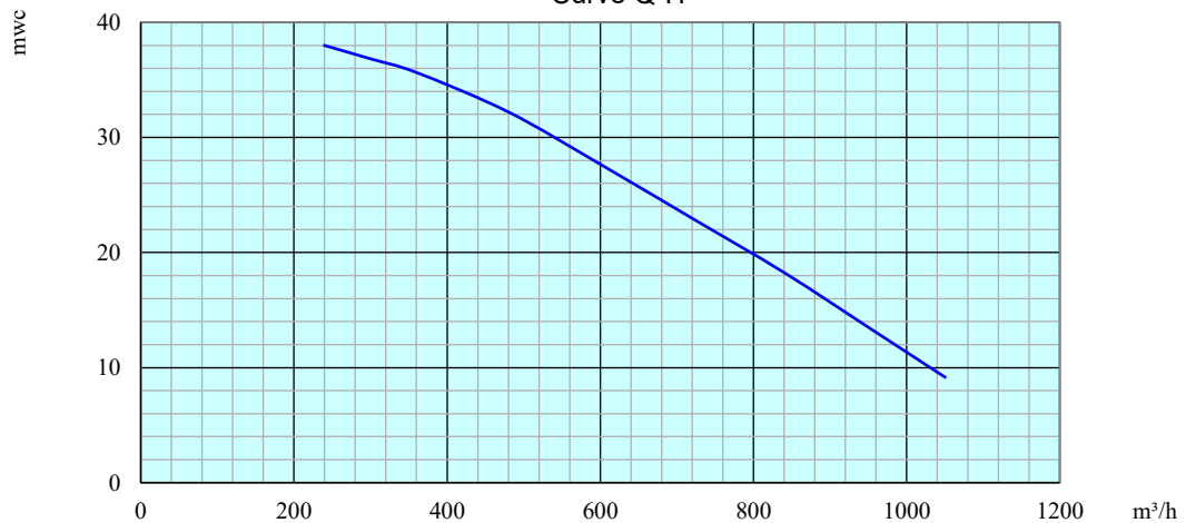
Curve Q-H
