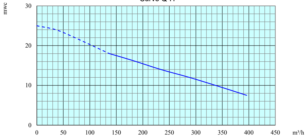
Curve Q-H
