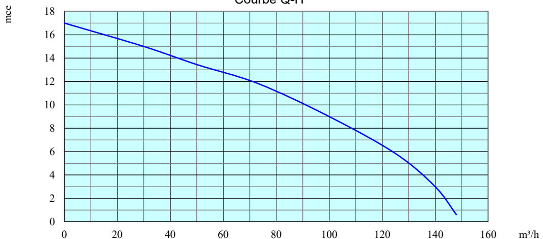
Courbe Q-H
