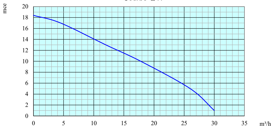
Courbe Q-H
