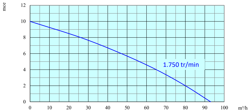
Courbe Q-H
