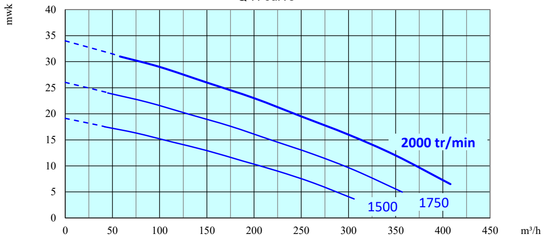
Q-H curve
