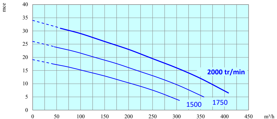
Courbe Q-H
