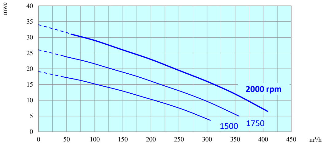
Q-H curve
