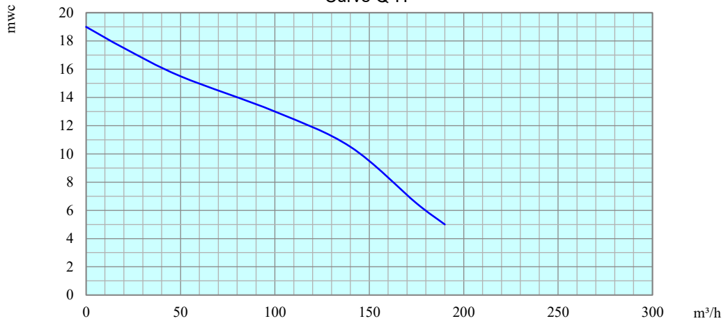
Curve Q-H
