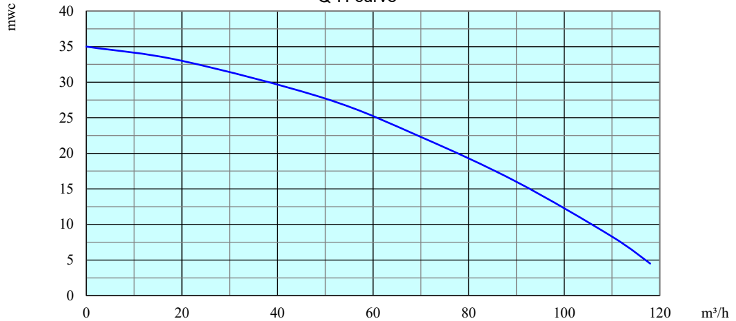
Q-H curve
