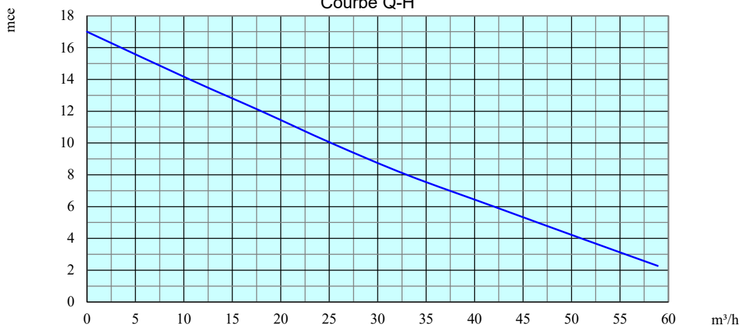
Courbe Q-H
