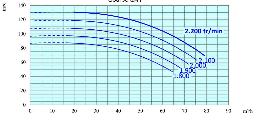
Courbe Q-H
