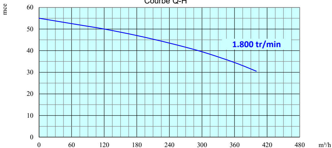
Courbe Q-H
