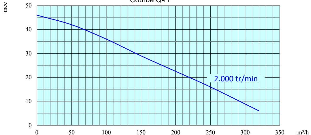
Courbe Q-H
