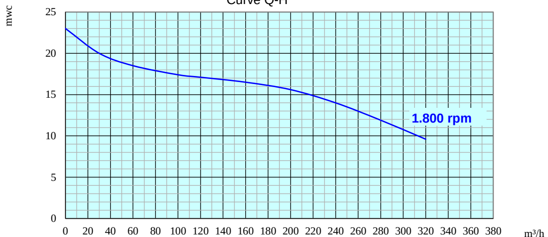
Curve Q-H
