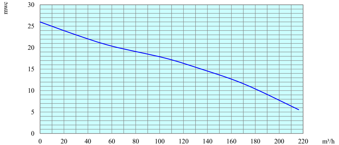
Curve Q-H
